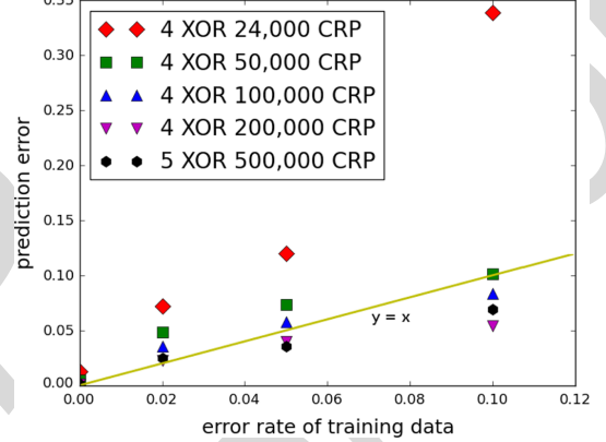
Fig. 7. Graphical illustration of the effect of error on LR in the training set, with chosen data points from Tables VI and VII. [Please cite Fig 7 in order in the text]
