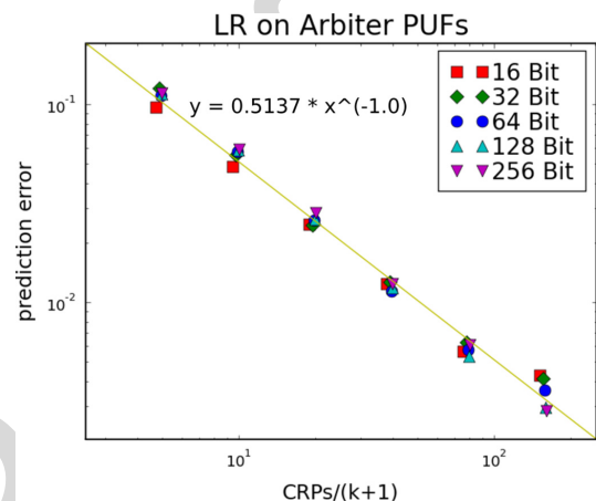
Fig. 1. Double logarithmic plot of misclassification rate \epsilon on the ratio of training CRPs N_{CRP} and \dim(\Phi) = k + 1 .
