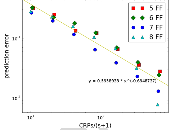
Fig. 6. Results of 10 trials per data point with ES for different numbers of FF-loops and the hyperbola fit.
