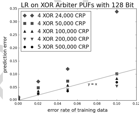
Fig. 7. Graphical illustration of the effect of error on LR in the training set, with chosen data points from Tables VI and VII. [Please cite Fig 7 in order in the text]
